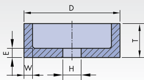
6 DxTxH-W..E.. Pages 44, 59
