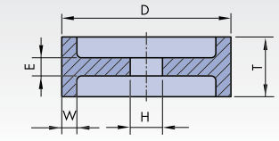
9 DxTxH-W..F..G.. Page 40
