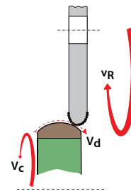
Diamond rolls
