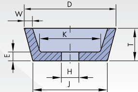
11 D/JxTxH-W..E..K.. Page 60
