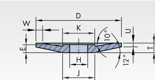
12BH D/JxT/UxH-WxExK-V..
