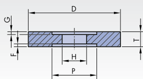
7 DxTxH-PxF/G Pages 40, 47, 49, 77, 93
