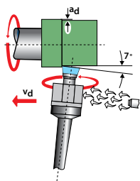
Dressing tools with rotating wings
